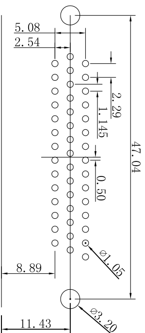
PCB layout
